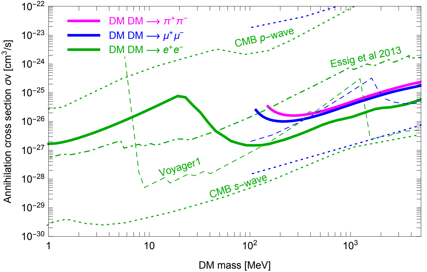
FIGURE 2: Our conservative constraints on sub-GeV DM from INTEGRAL data (solid thick lines), compared to other existing bounds: from VOYAGER 1 e^\pm data (dashed green and blue lines, from Boudaud et al. [26]), from a compilation of X-ray data (dot-dashed green line, from Essig et al. [43]), and from the CMB assuming s -wave (dotted green and blue lines in the lower portion of the plot, from Slatyer [45] and Lopez-Honorez et al. [46]) or p -wave annihilation (dotted green and blue lines in the upper portion of the plot, from Diamanti et al. [49] and Liu et al. [50]); these bounds are rescaled up by a factor (v/v_{\text{ref}})^2 = (220/100)^2 since they are provided in the literature for v_{\text{ref}} = 100 km/s while we consider v \simeq 220 km/s in the Milky Way). For each probe, we use the color code specified in the legend: green for the \text{DM DM} \rightarrow e^+e^- annihilation channel, blue for \text{DM DM} \rightarrow \mu^+\mu^- and magenta for \text{DM DM} \rightarrow \pi^+\pi^- . When results on a channel are not present in the literature, the corresponding color is missing. For instance, there are no bounds from these probes on the \pi^+\pi^- channel besides ours.
