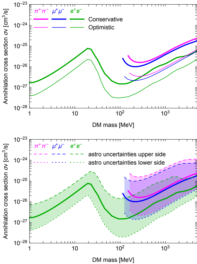
FIGURE 3: Impact of the methodology and the uncertainties on the constraints. Top panel: constraints with and without astrophysical background. Bottom panel: variation of the bounds due to the astrophysical uncertainties.
