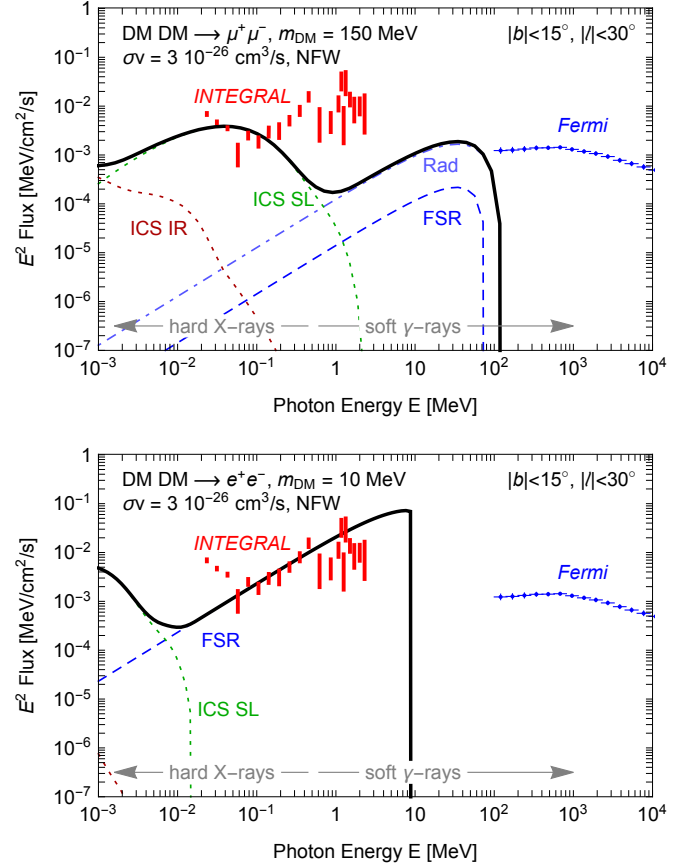
FIGURE 1: Example photon spectra from sub-GeV DM, which illustrate our main points. Top panel: the hard X-ray and soft \gamma -ray spectrum produced by a 150 MeV DM particle annihilating into \mu^+\mu^- . We show the different components in color and the total flux in thick black. The spectrum cuts off before reaching FERMI’s data (taken from [44] and reported here just for reference, as they are not the focus of our work) but produces a signal in X-rays that can be constrained by INTEGRAL (taken from [39], Figure 7). The Final State Radiation (FSR, blue dashed) and Radiative Decay (Rad, blue dot-dashed) contributions yield signals that pass well below the X-ray data. However, the inclusion of the DM-induced Inverse Compton Scattering (ICS) contribution on the different components of the Galactic ambient light (starlight (SL, green dotted), dust-reprocessed infrared light (IR, brown dotted)) and the CMB (not visible in the plot), leads to a flux which is orders of magnitude larger, thus producing stronger constraints. Bottom panel: the same for a 10 MeV DM particle annihilating into e^+e^- . In this case, the limit is instead driven by the FSR contribution because the DM ICS contributions fall to too low energy for INTEGRAL. In these illustrations, the signals are computed over the |b| < 15^\circ , |\ell| < 30^\circ region of interest (RoI): in our analysis, we actually use smaller RoIs, removing low latitudes.
